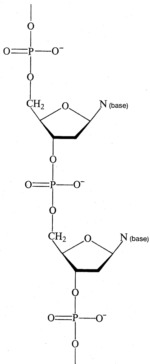
DNA
