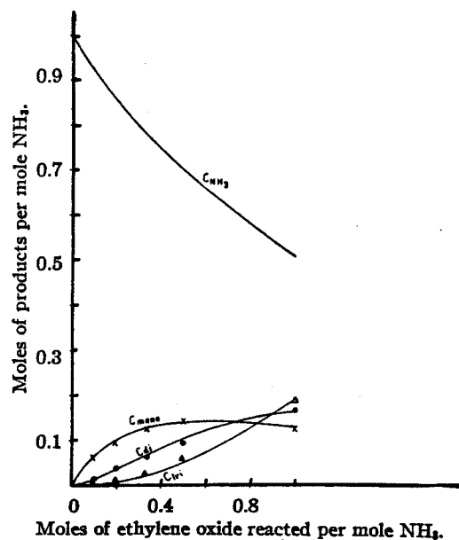
Fig. 2.—Distribution of products in ethanolamines synthesis. Batch process at 15°; —, calcd. curves; X O Δ □, exptl. values.
