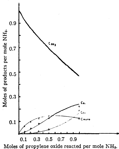
Fig. 3.—Distribution of products in isopropanolamines synthesis. Batch process at 15°: —, calcd. curves; X \odot \Delta , exptl. values.
