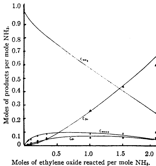
Fig. 4.—Distribution of products in ethanolamines synthesis. Continuous process at 15°: —, calcd. curves; X \odot \Delta , exptl. values.
